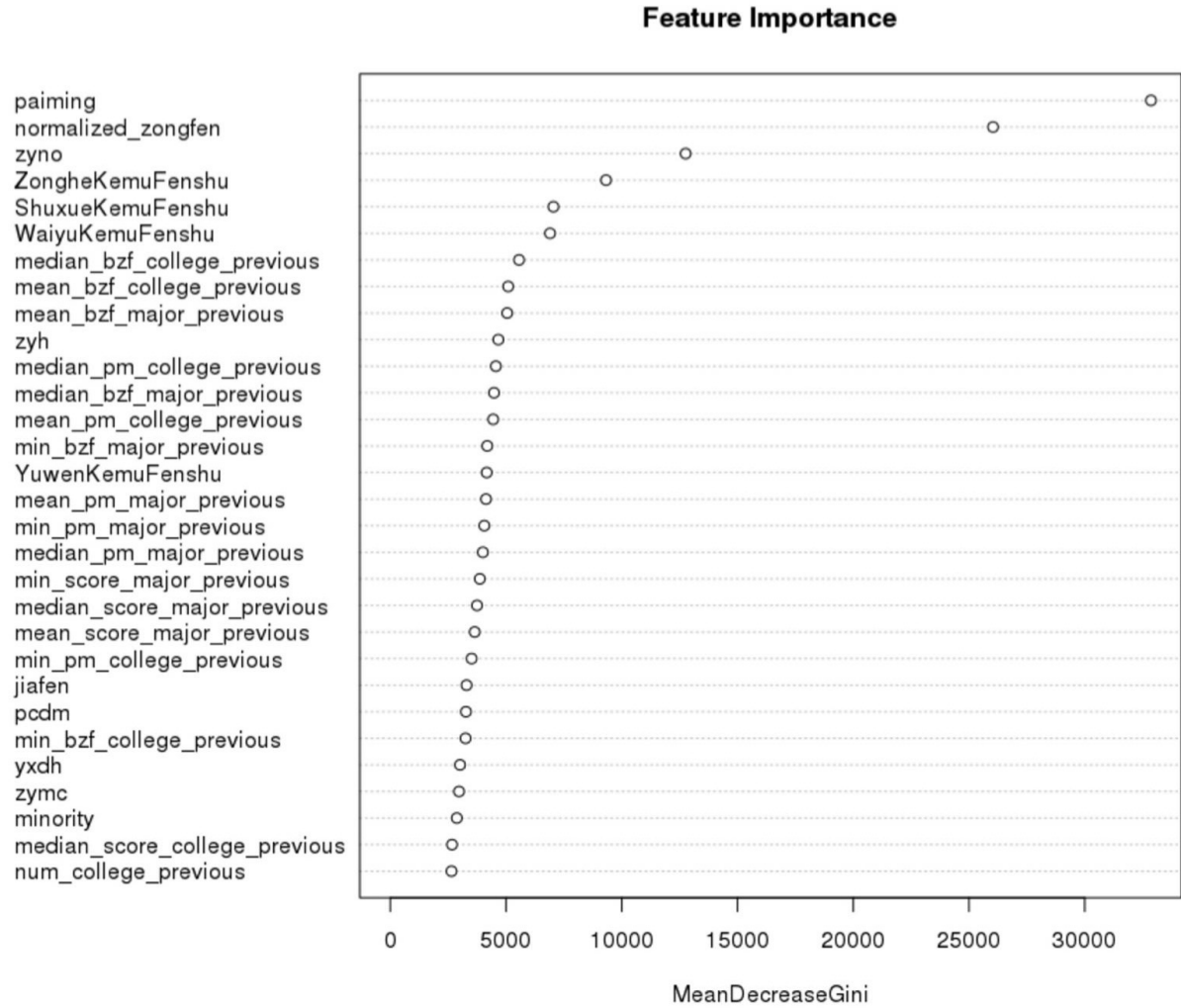
Figure A.3: Relative importance of features in the random forest predictions
